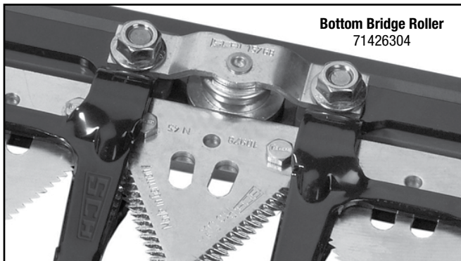
Bottom Bridge Roller reduces vibration and wear of knifeback
