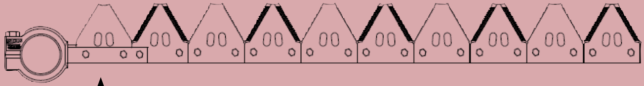
Full Section on Drive End of Knife
