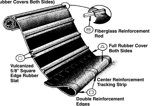
HEAVY DUTY (Rubber Covers Both Sides)
