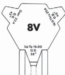
Sheave Groove Gauge
