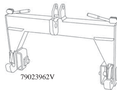
Category 2/3 Quick Hitch
